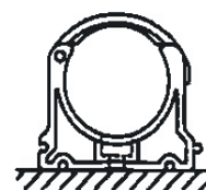
Assembly situation A Mounting on the floor
