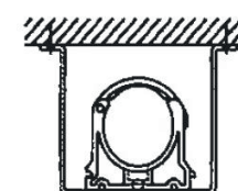
Assembly situation C Mounting on the ceiling supported horizontally
